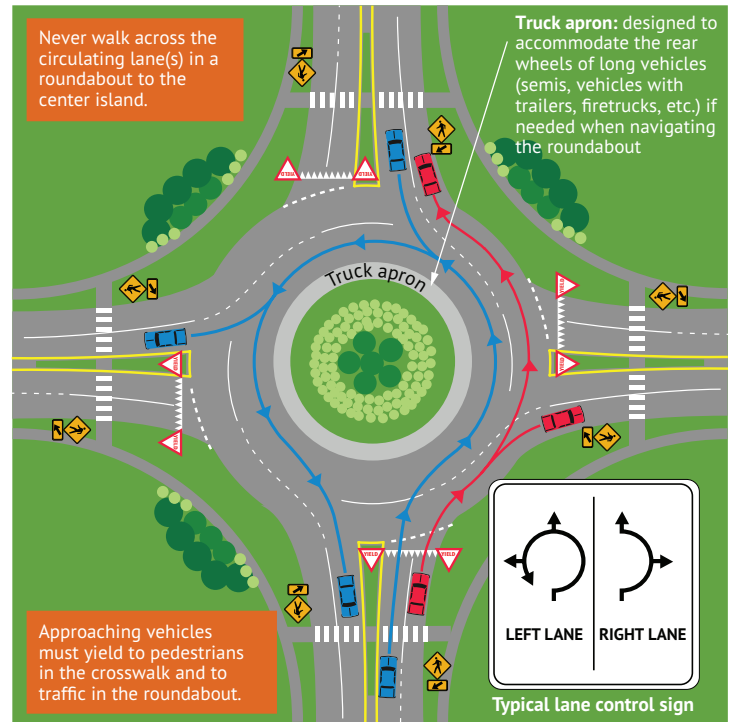
Figure 5.5: Multi-lane roundabout
