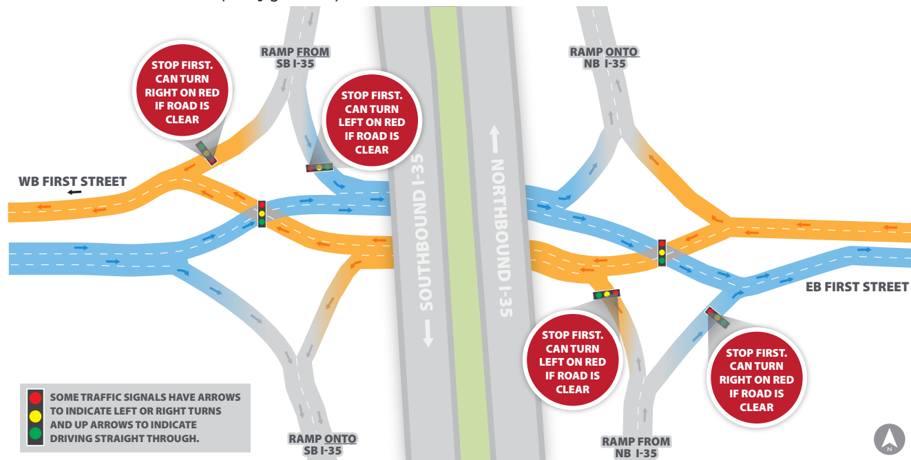
Figure 5.3: Diverging diamond interchange (Example shows the I-35 and First Street diverging diamond interchange in Ankeny.)
