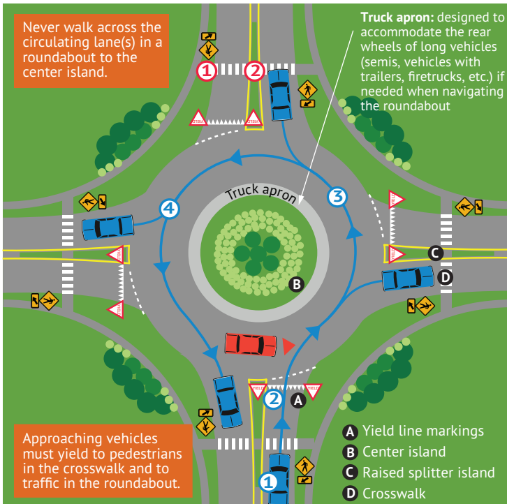
Figure 5.4: Single-lane roundabout
